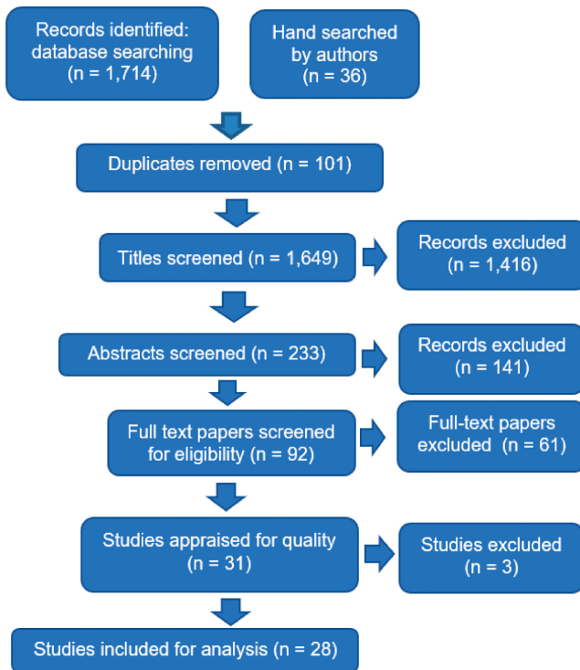
Figure 1. STUDY SELECTION
