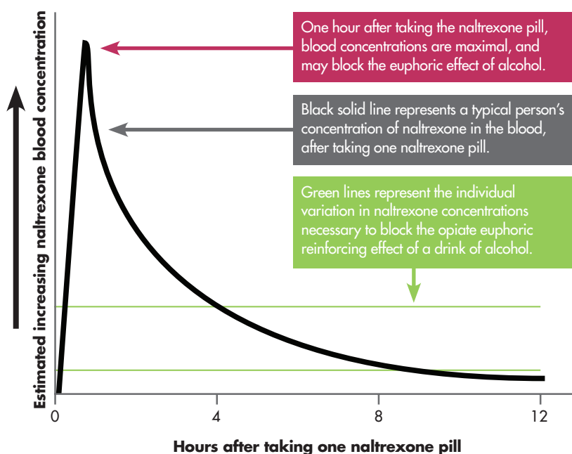
FIGURE 2: Naltrexone blood concentration level
